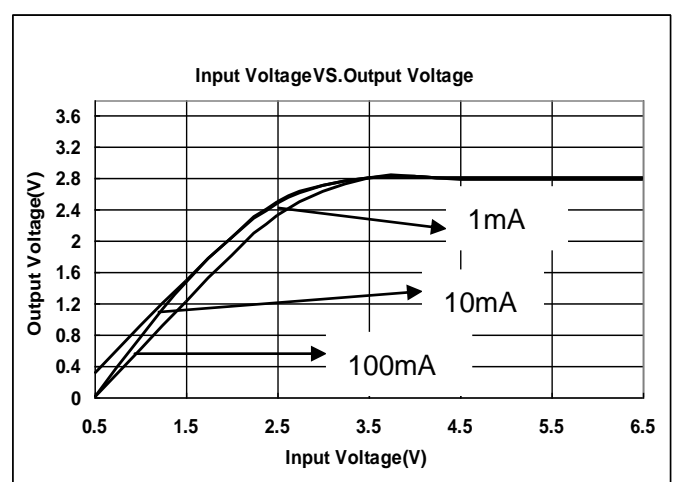
ME6206A28PG
